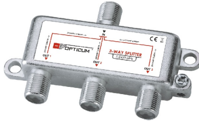
3-WAY SPLITTER
